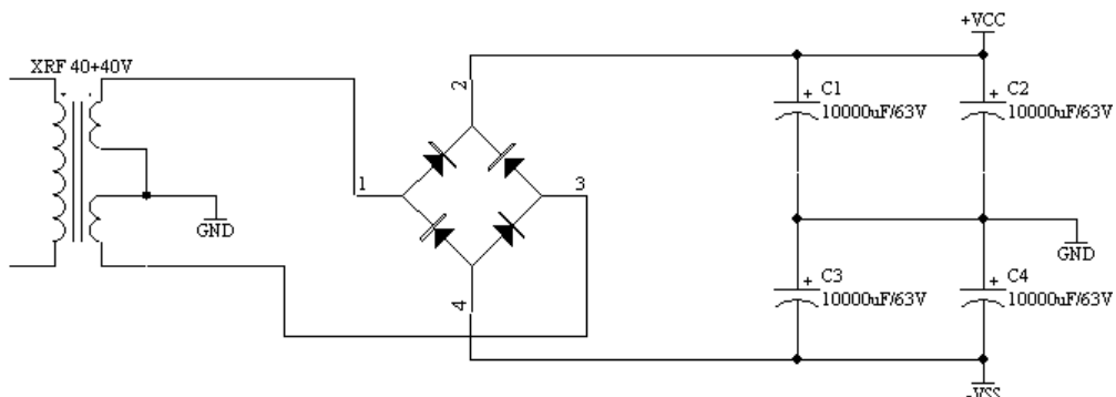
Fig.2: Example of linear power supply arrangement for the BP4078
